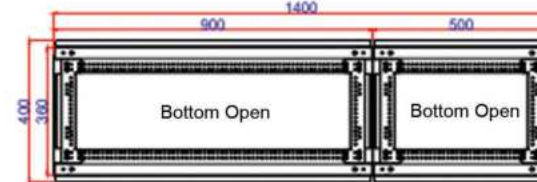
Bottom View
