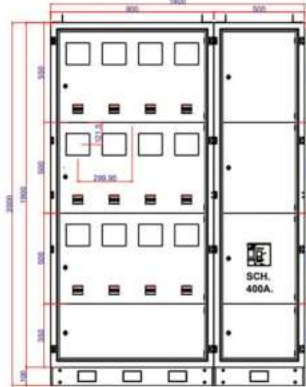
Cover Front View
